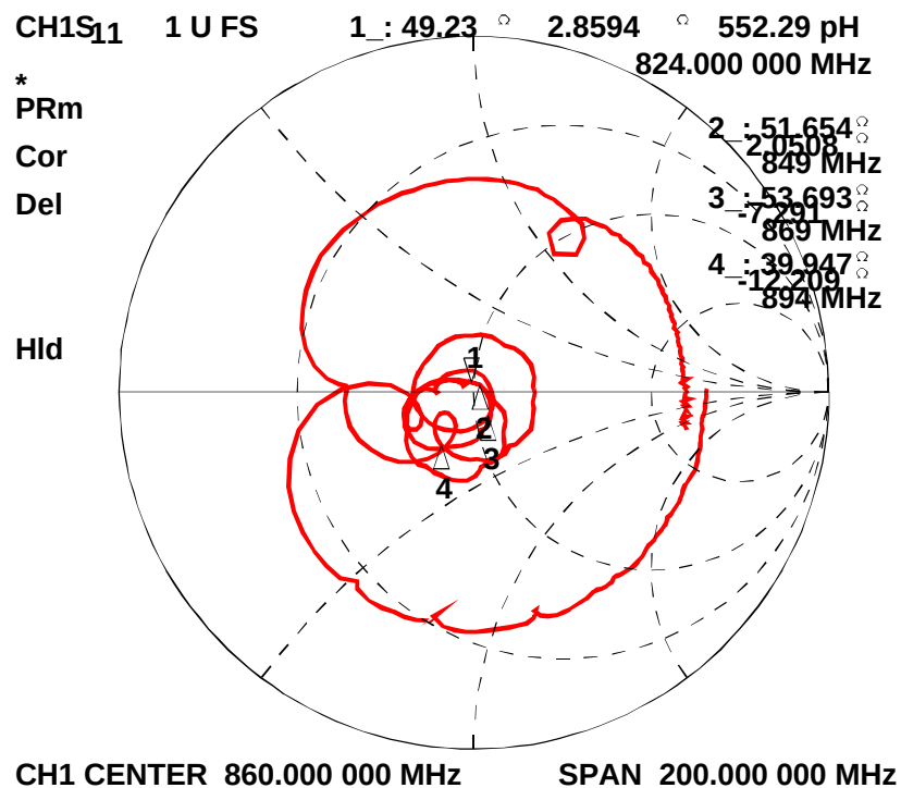
Figure 3-4 Electrical Characteristics
