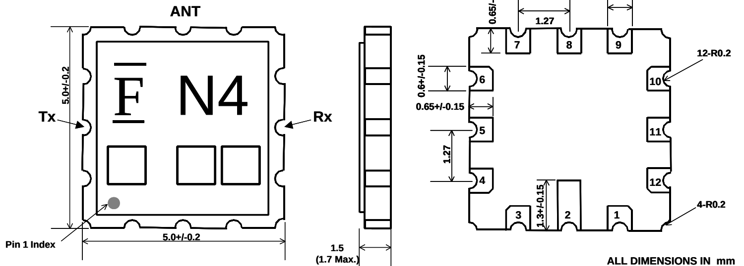
TOP VIEW
